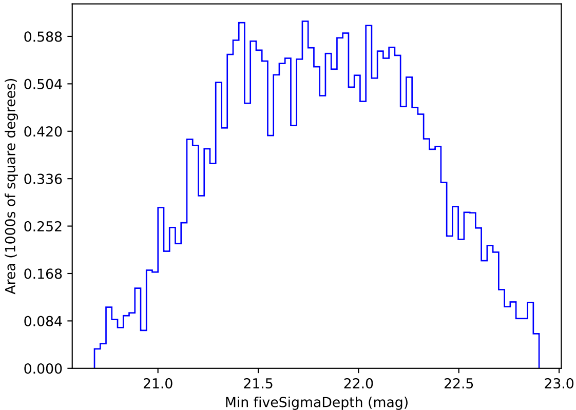
mw_roll_all_v3.3_10yrs All sky i band: Min fiveSigmaDepth
