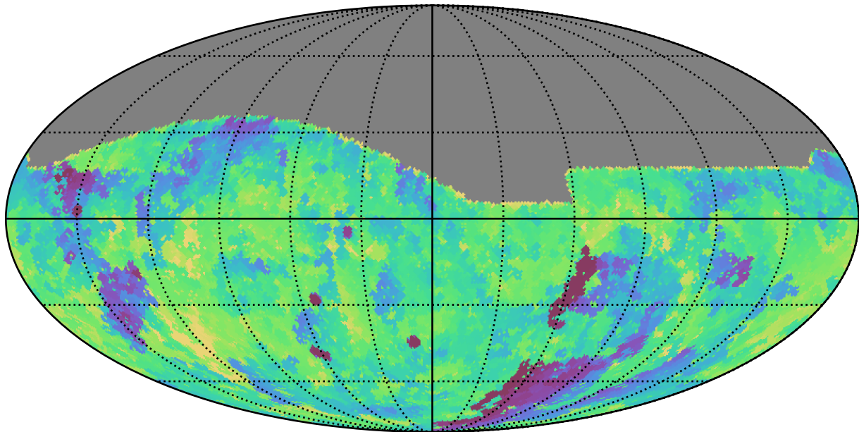
mw_roll_all_v3.3_10yrs All sky g band: Min fiveSigmaDepth
