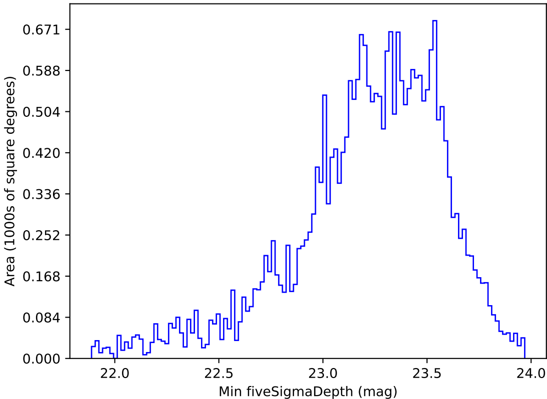
mw_roll_all_v3.3_10yrs All sky g band: Min fiveSigmaDepth
