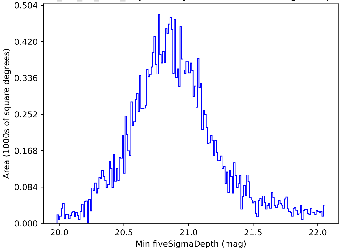
mw_roll_all_v3.3_10yrs All sky all bands: Min fiveSigmaDepth
