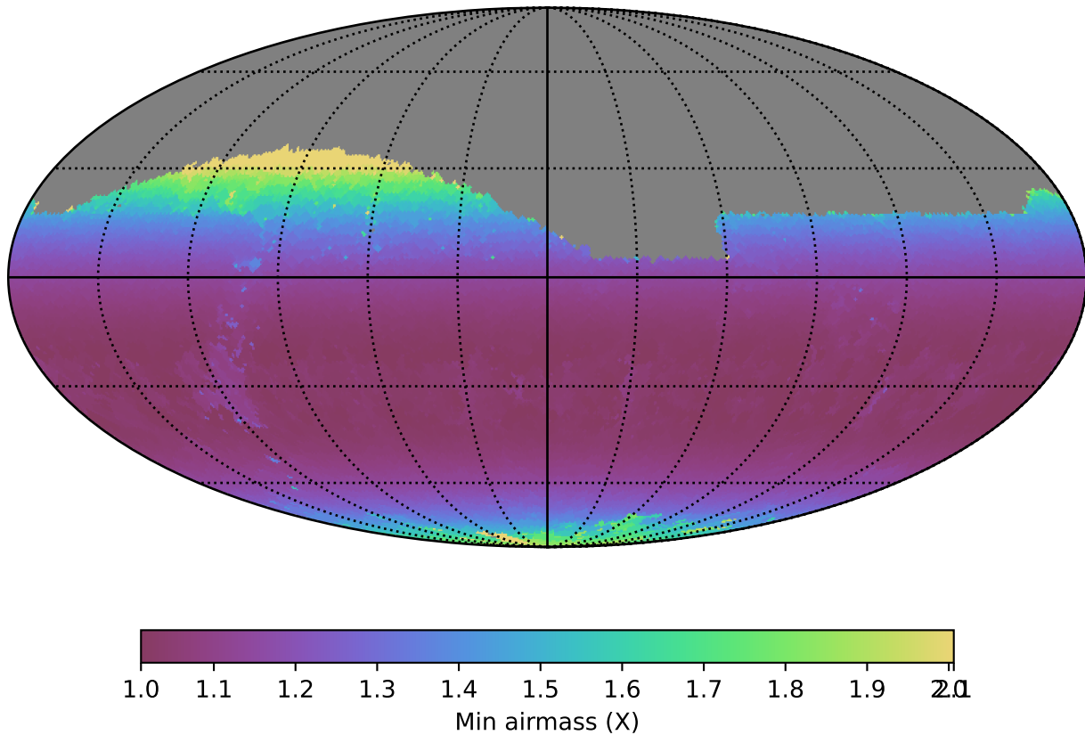
mw_roll_all_v3.3_10yrs Yr 1 z band: Min airmass
