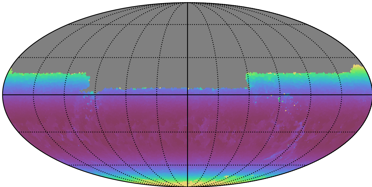
mw_roll_all_v3.3_10yrs Yr 1 y band: Min airmass
