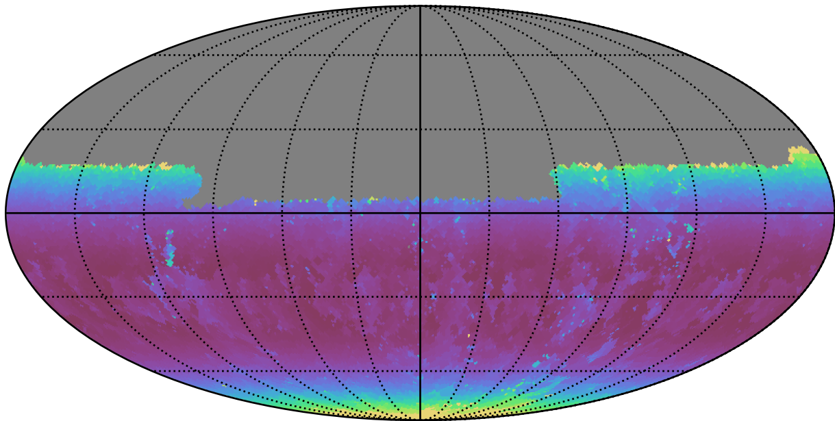
mw_roll_all_v3.3_10yrs Yr 1 u band: Min airmass
