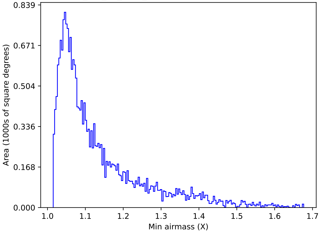
mw_roll_all_v3.3_10yrs Yr 1 u band: Min airmass
