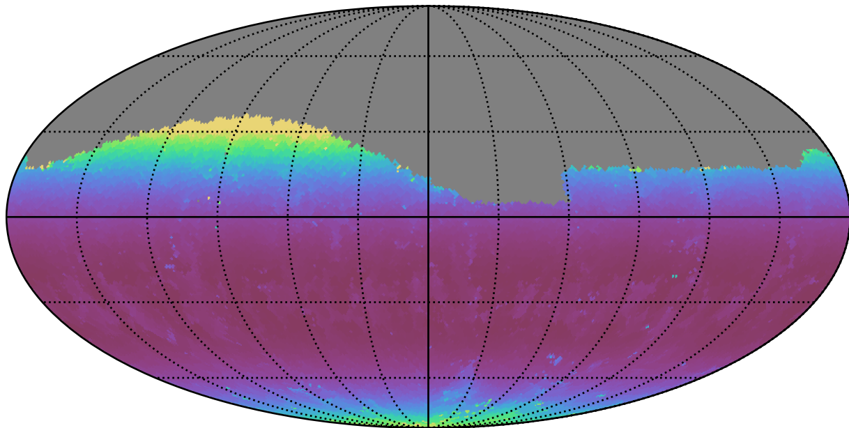
mw_roll_all_v3.3_10yrs Yr 1 g band: Min airmass
