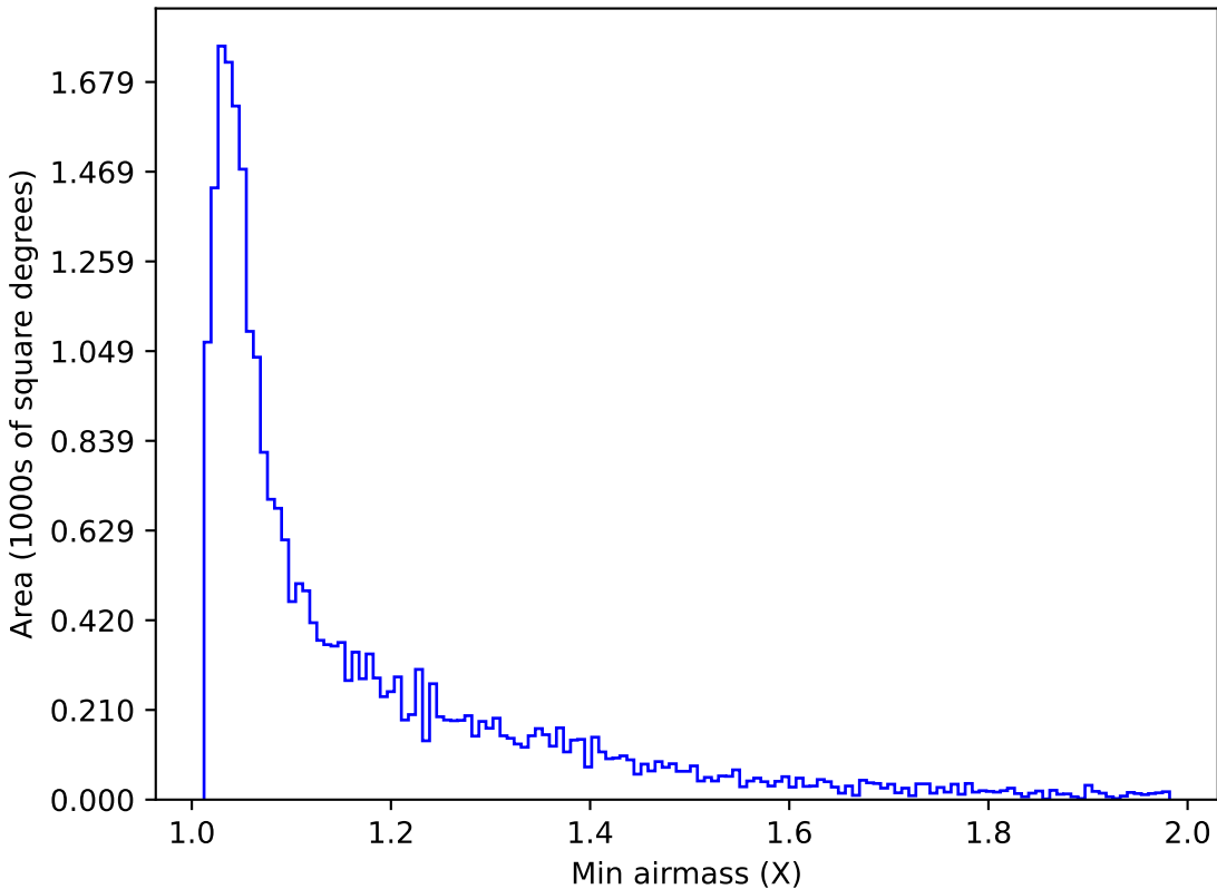
mw_roll_all_v3.3_10yrs Yr 1 g band: Min airmass
