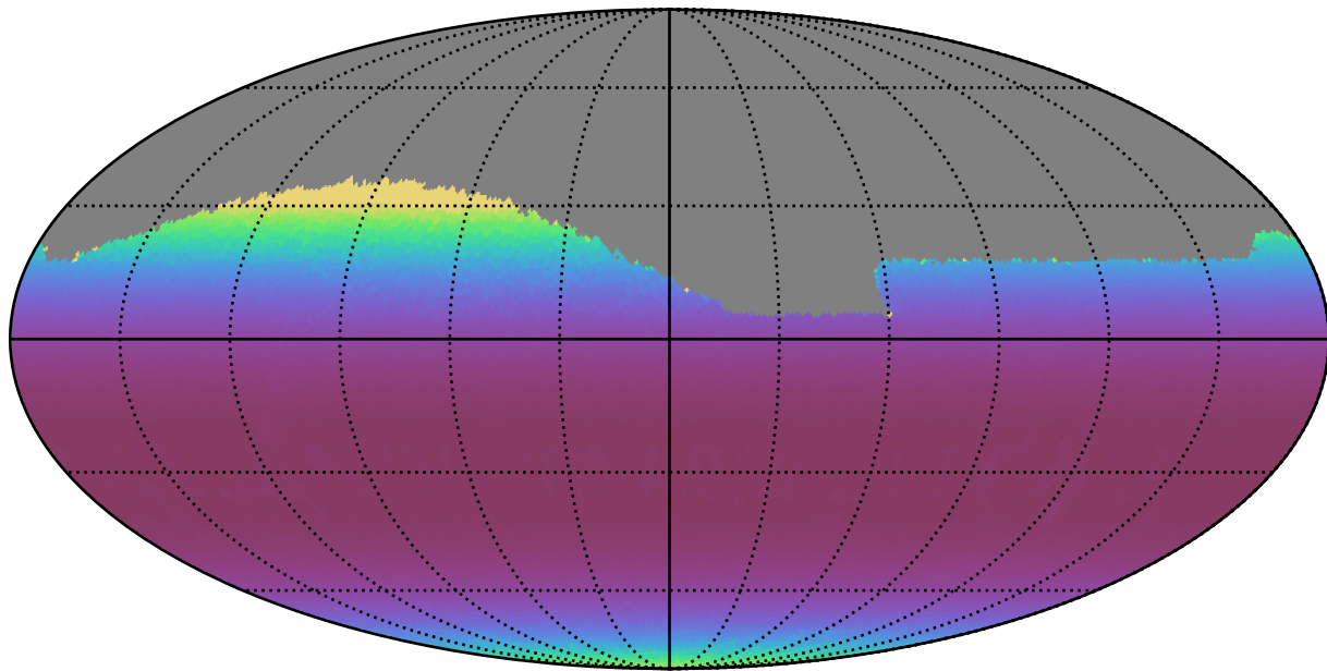
mw_roll_all_v3.3_10yrs Yr 1 all bands: Min airmass
