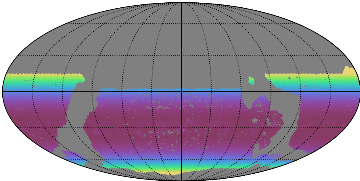
mw_roll_all_v3.3_10yrs WFD z band: Min airmass
