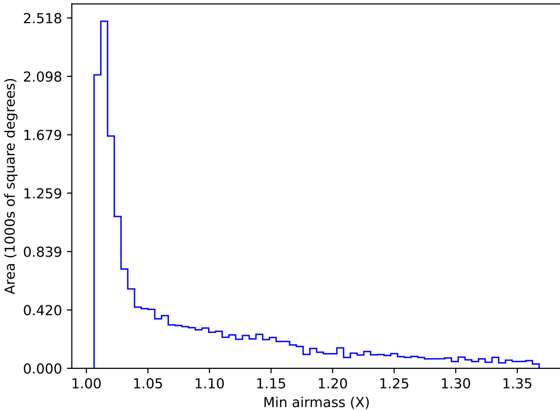
mw_roll_all_v3.3_10yrs WFD z band: Min airmass
