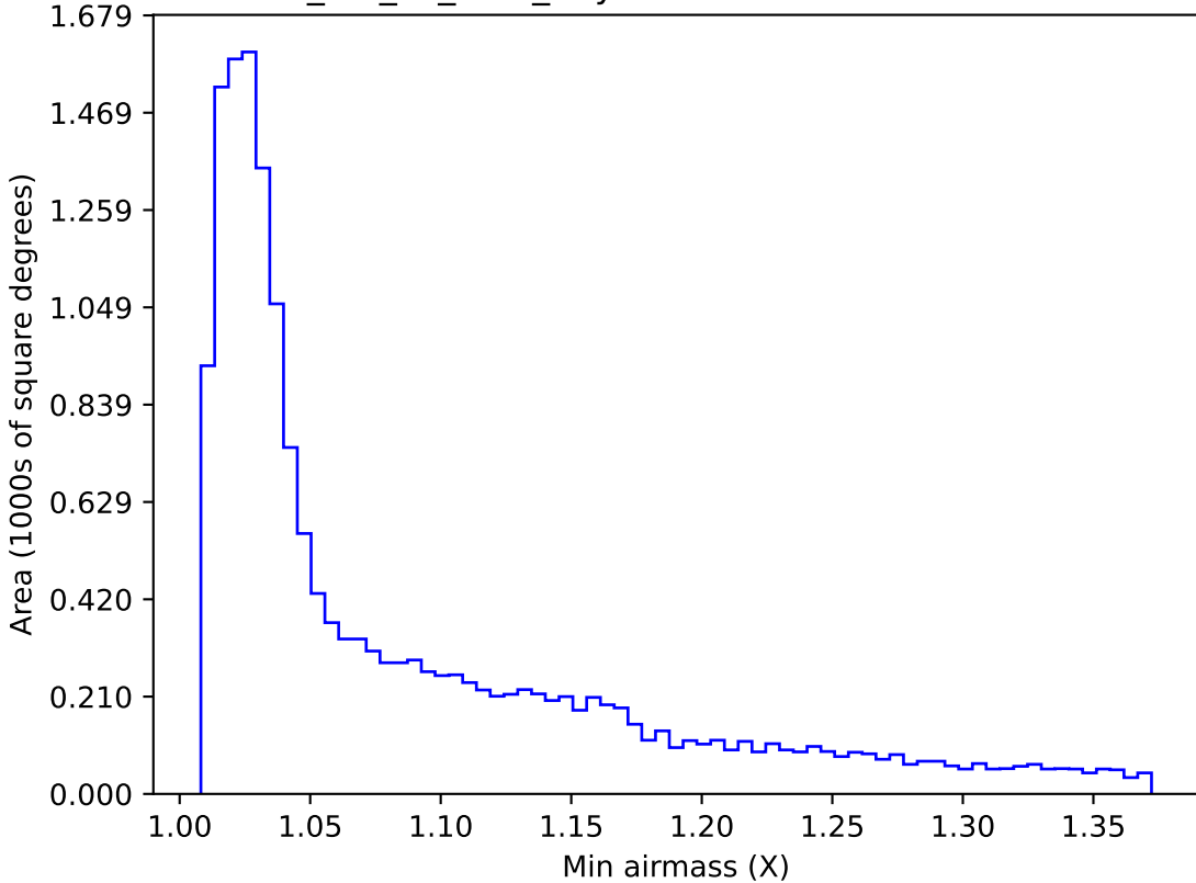
mw_roll_all_v3.3_10yrs WFD u band: Min airmass
