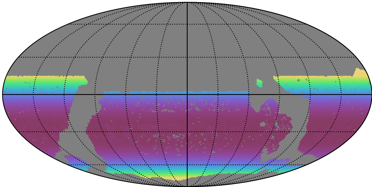
mw_roll_all_v3.3_10yrs WFD r band: Min airmass
