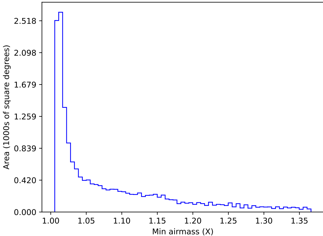
mw_roll_all_v3.3_10yrs WFD r band: Min airmass
