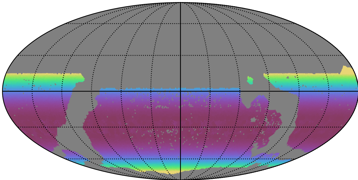
mw_roll_all_v3.3_10yrs WFD i band: Min airmass
