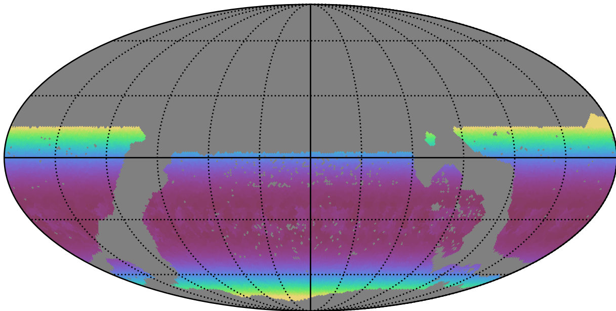
mw_roll_all_v3.3_10yrs WFD g band: Min airmass
