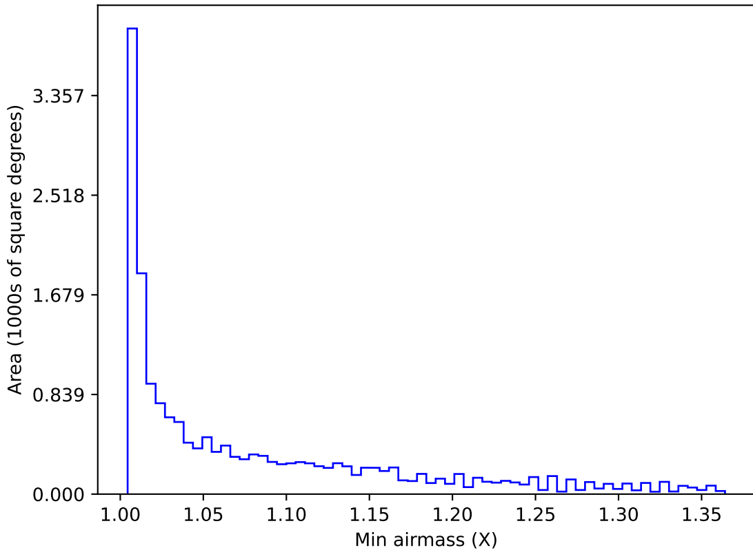
mw_roll_all_v3.3_10yrs WFD all bands: Min airmass
