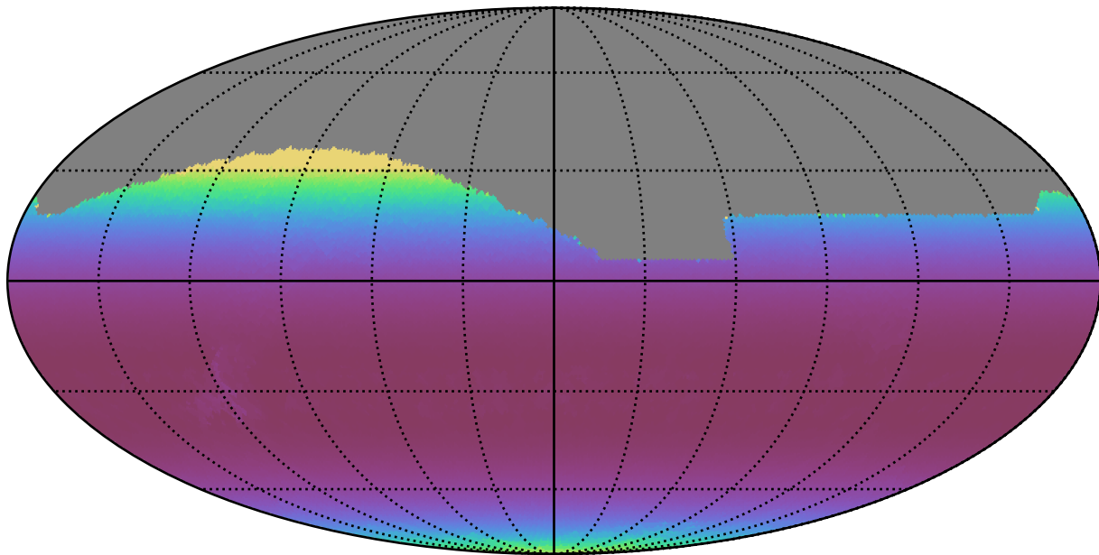
mw_roll_all_v3.3_10yrs All sky z band: Min airmass
