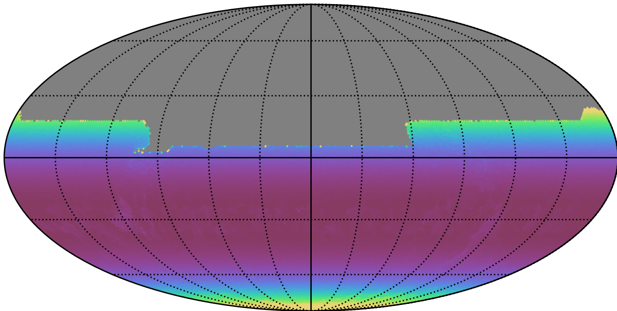
mw_roll_all_v3.3_10yrs All sky y band: Min airmass
