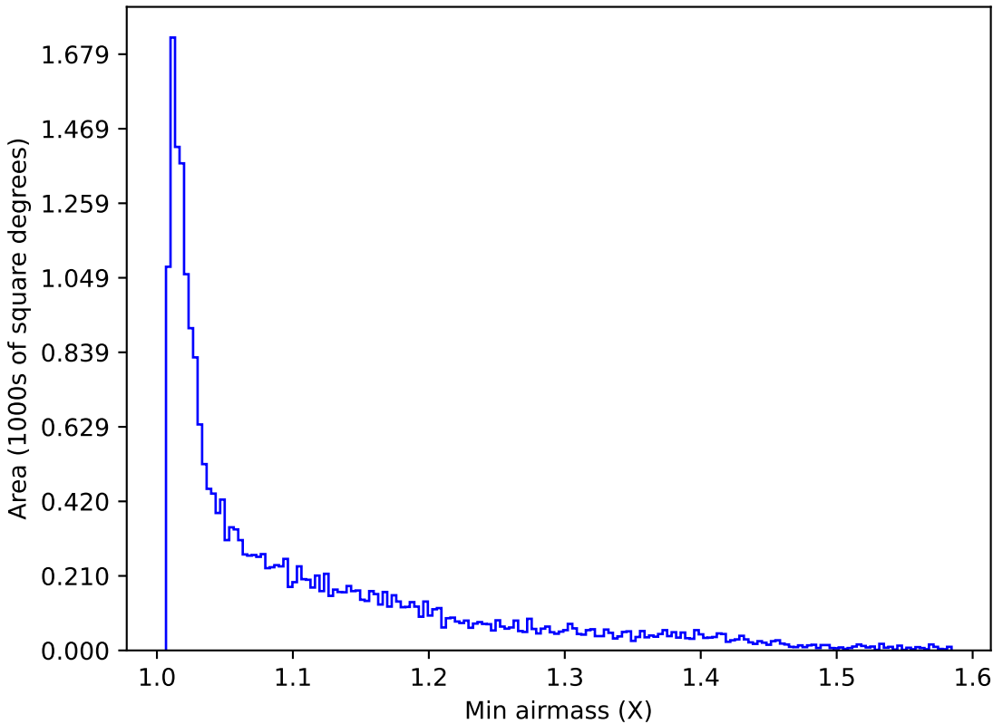
mw_roll_all_v3.3_10yrs All sky y band: Min airmass
