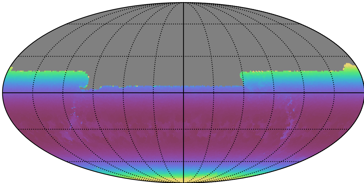
mw_roll_all_v3.3_10yrs All sky u band: Min airmass
