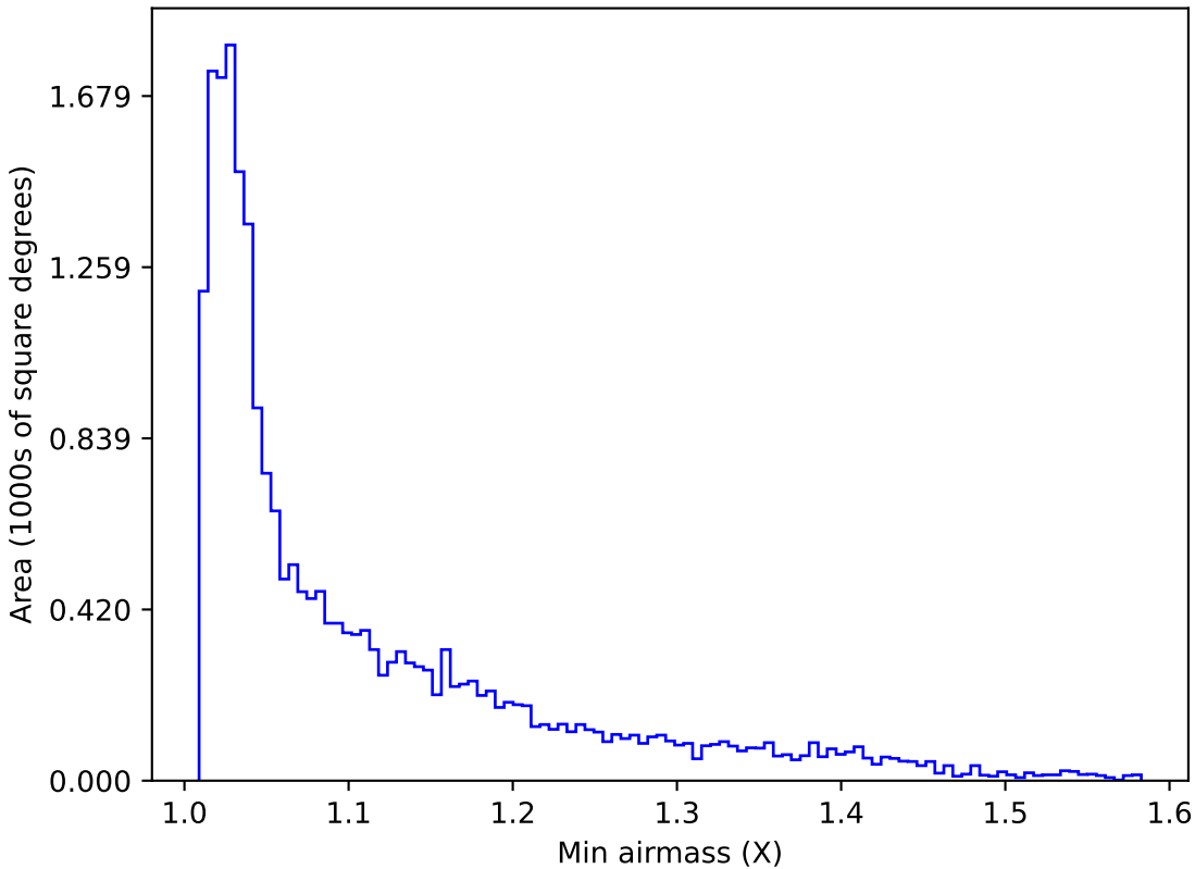
mw_roll_all_v3.3_10yrs All sky u band: Min airmass
