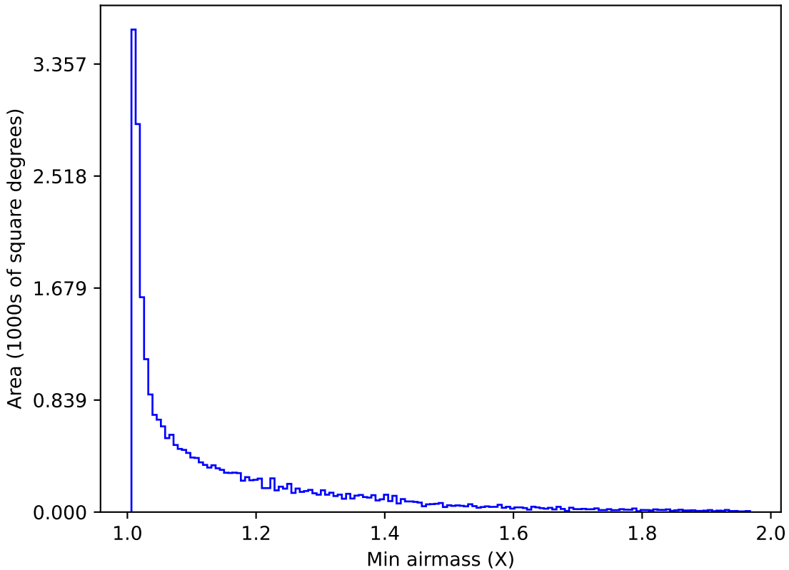
mw_roll_all_v3.3_10yrs All sky r band: Min airmass
