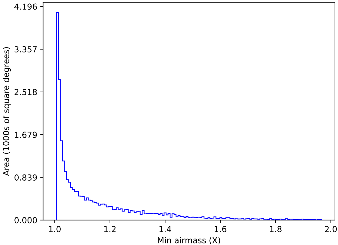
mw_roll_all_v3.3_10yrs All sky i band: Min airmass
