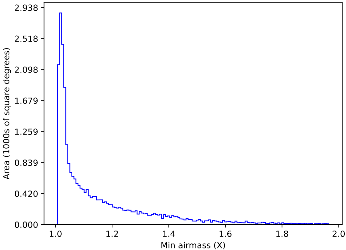
mw_roll_all_v3.3_10yrs All sky g band: Min airmass
