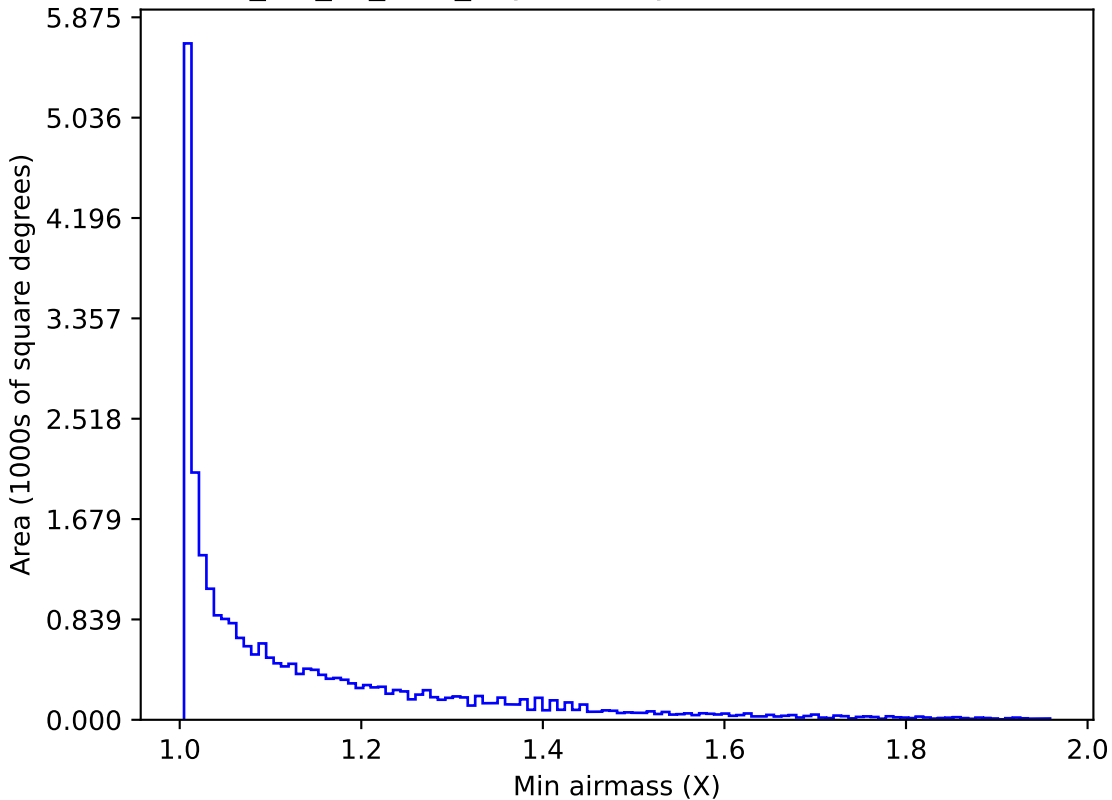
mw_roll_all_v3.3_10yrs All sky all bands: Min airmass
