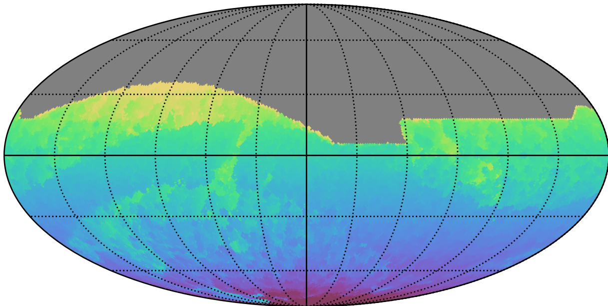
mw_roll_all_v3.3_10yrs All sky all bands: Min HA
