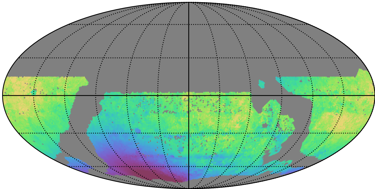
mw_roll_all_v3.3_10yrs WFD z band: Median solarElong
