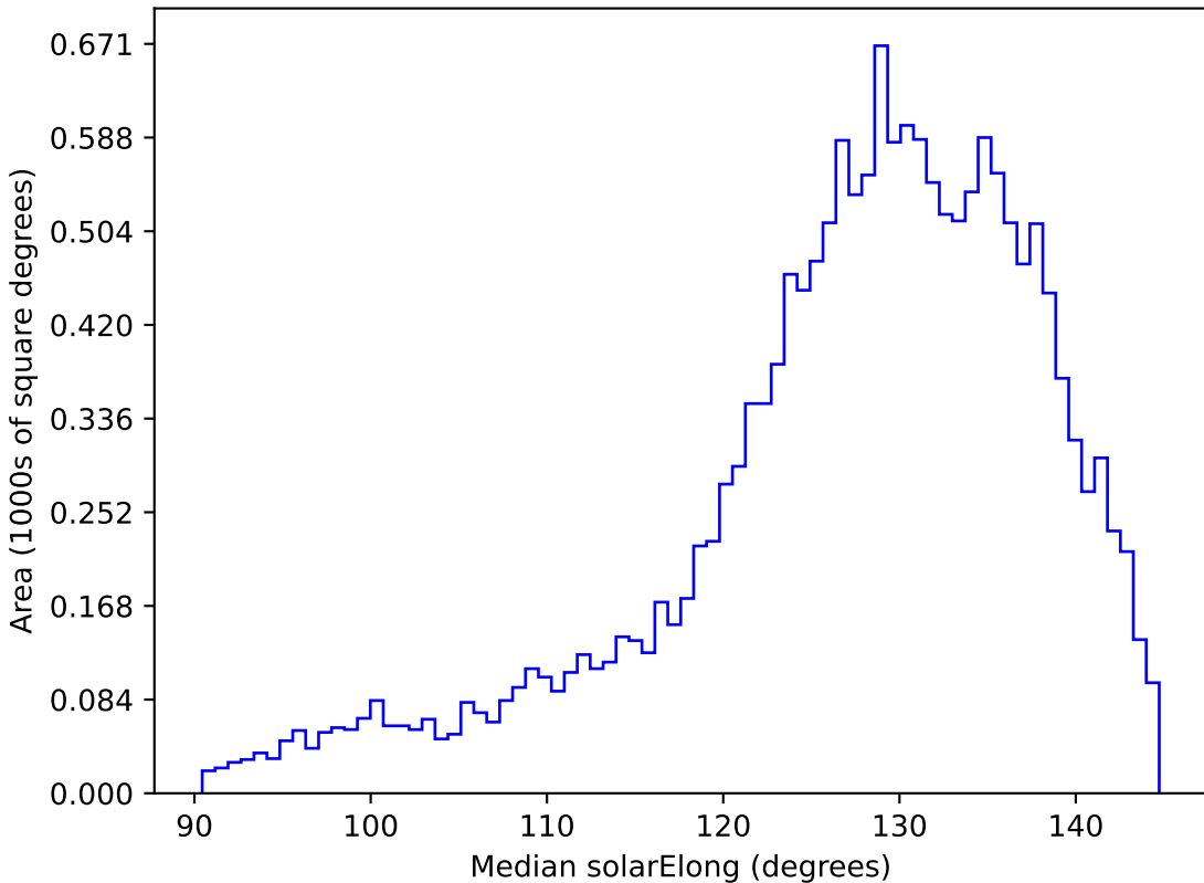
mw_roll_all_v3.3_10yrs WFD z band: Median solarElong
