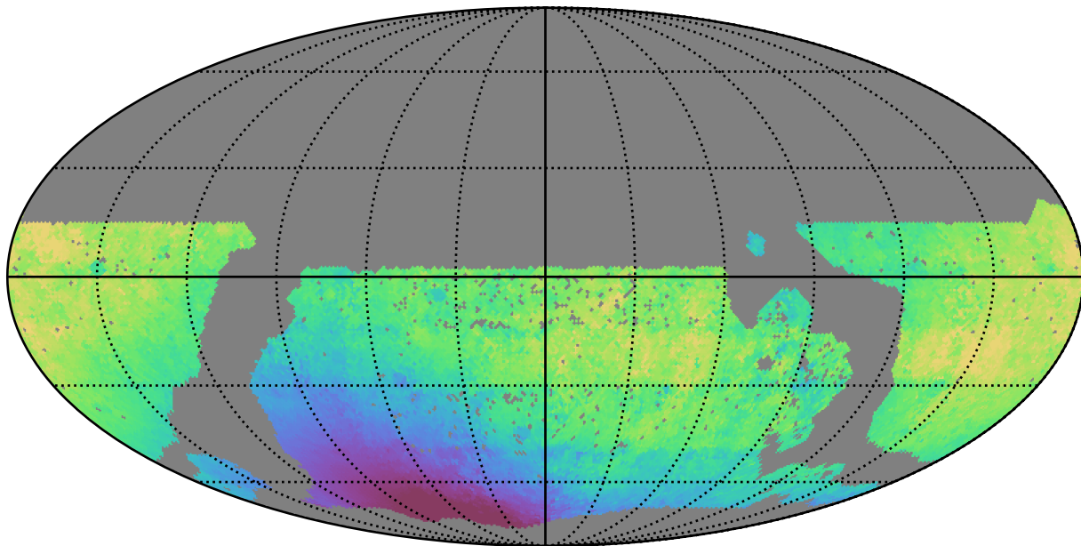
mw_roll_all_v3.3_10yrs WFD y band: Median solarElong
