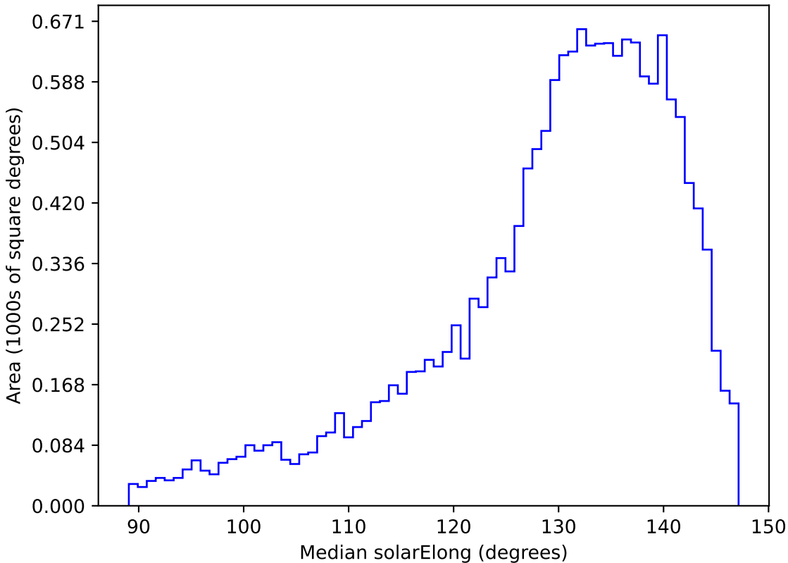
mw_roll_all_v3.3_10yrs WFD y band: Median solarElong
