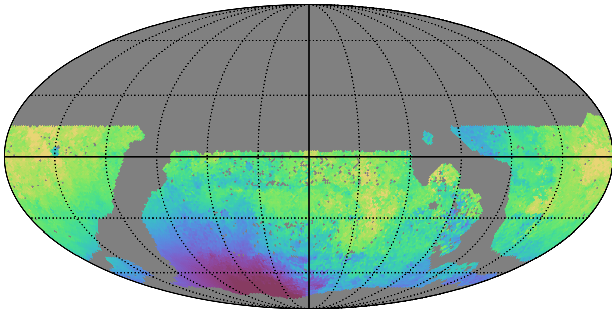
mw_roll_all_v3.3_10yrs WFD u band: Median solarElong
