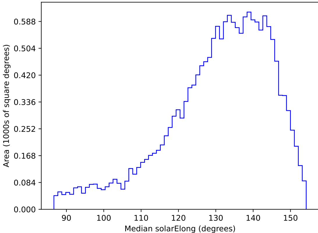
mw_roll_all_v3.3_10yrs WFD u band: Median solarElong
