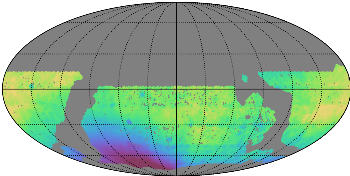
mw_roll_all_v3.3_10yrs WFD r band: Median solarElong
