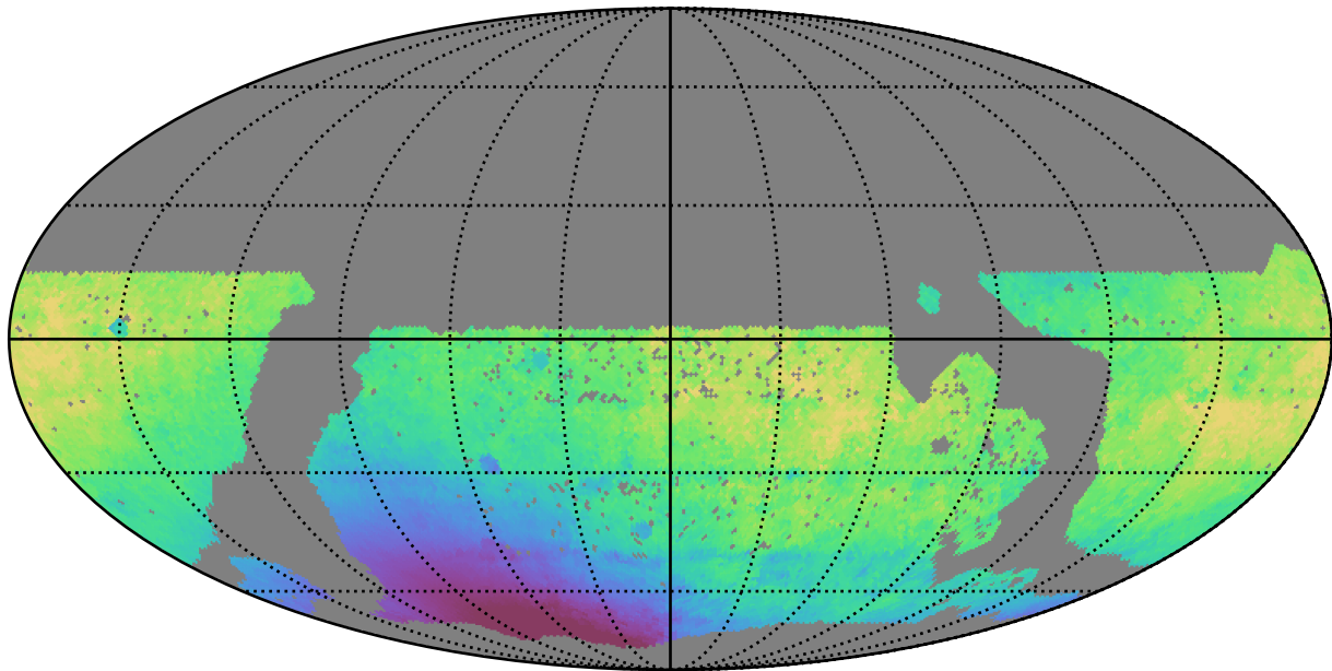
mw_roll_all_v3.3_10yrs WFD i band: Median solarElong
