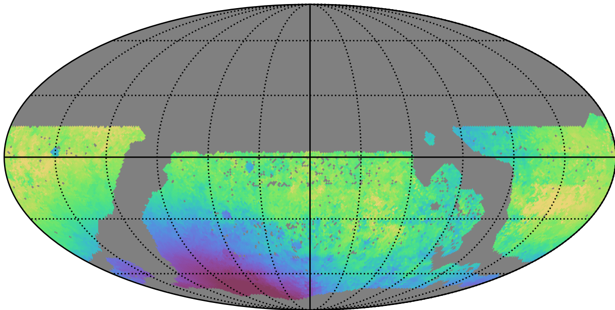
mw_roll_all_v3.3_10yrs WFD g band: Median solarElong
