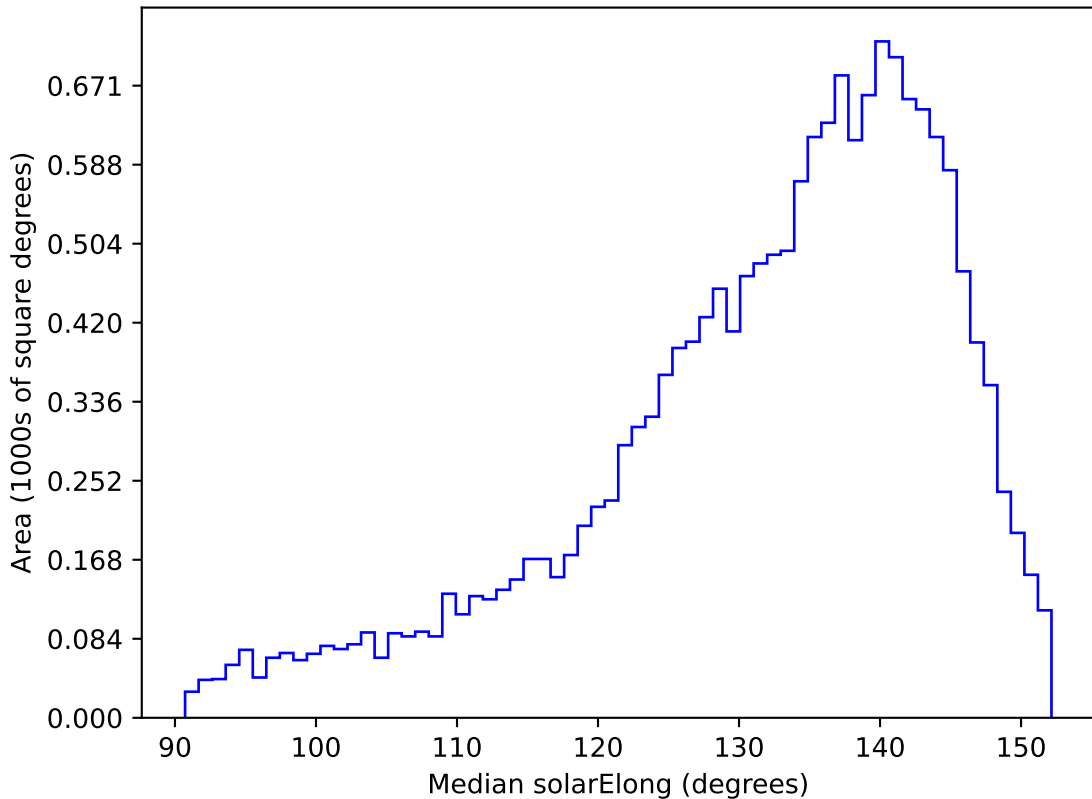
mw_roll_all_v3.3_10yrs WFD g band: Median solarElong
