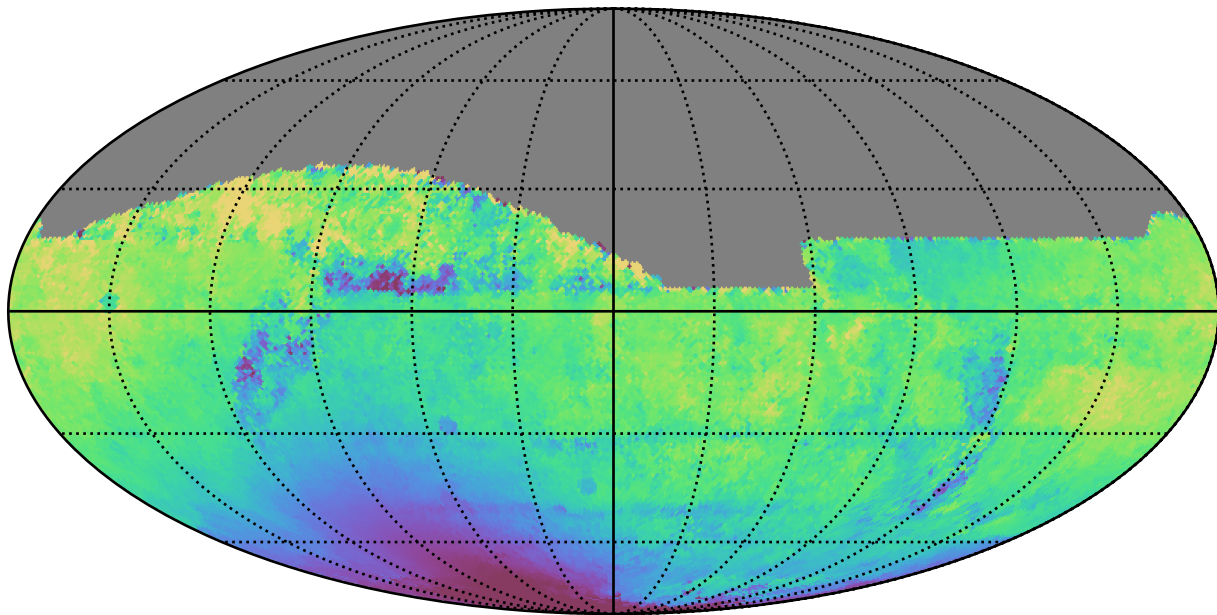
mw_roll_all_v3.3_10yrs All sky z band: Median solarElong
