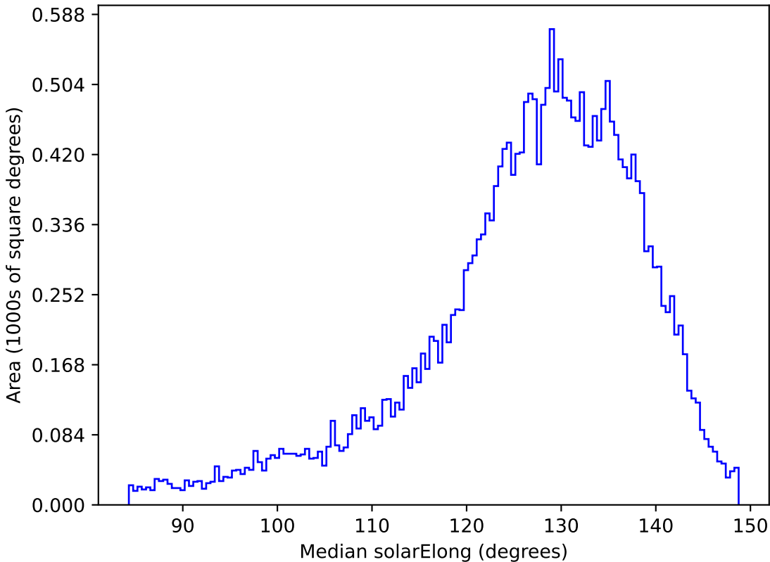
mw_roll_all_v3.3_10yrs All sky z band: Median solarElong
