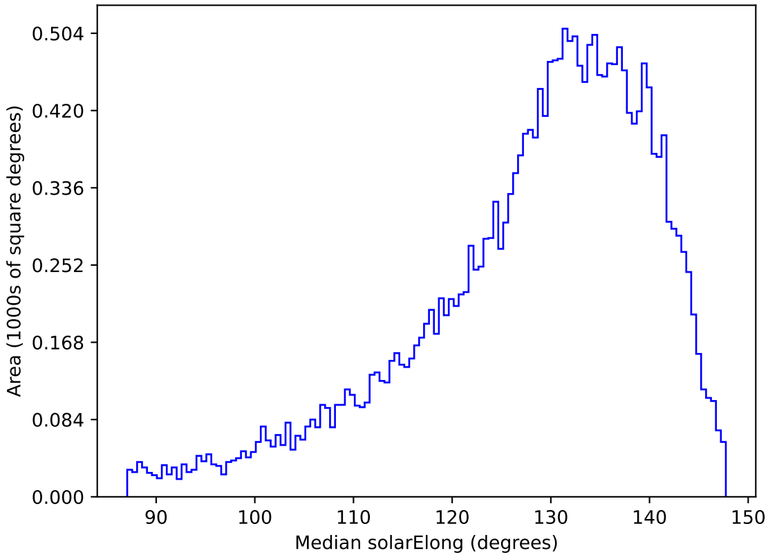
mw_roll_all_v3.3_10yrs All sky y band: Median solarElong
