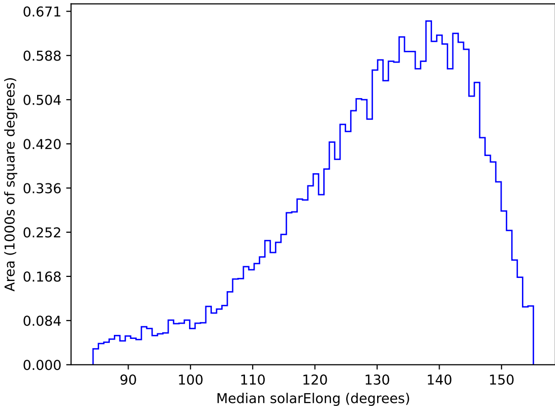
mw_roll_all_v3.3_10yrs All sky u band: Median solarElong
