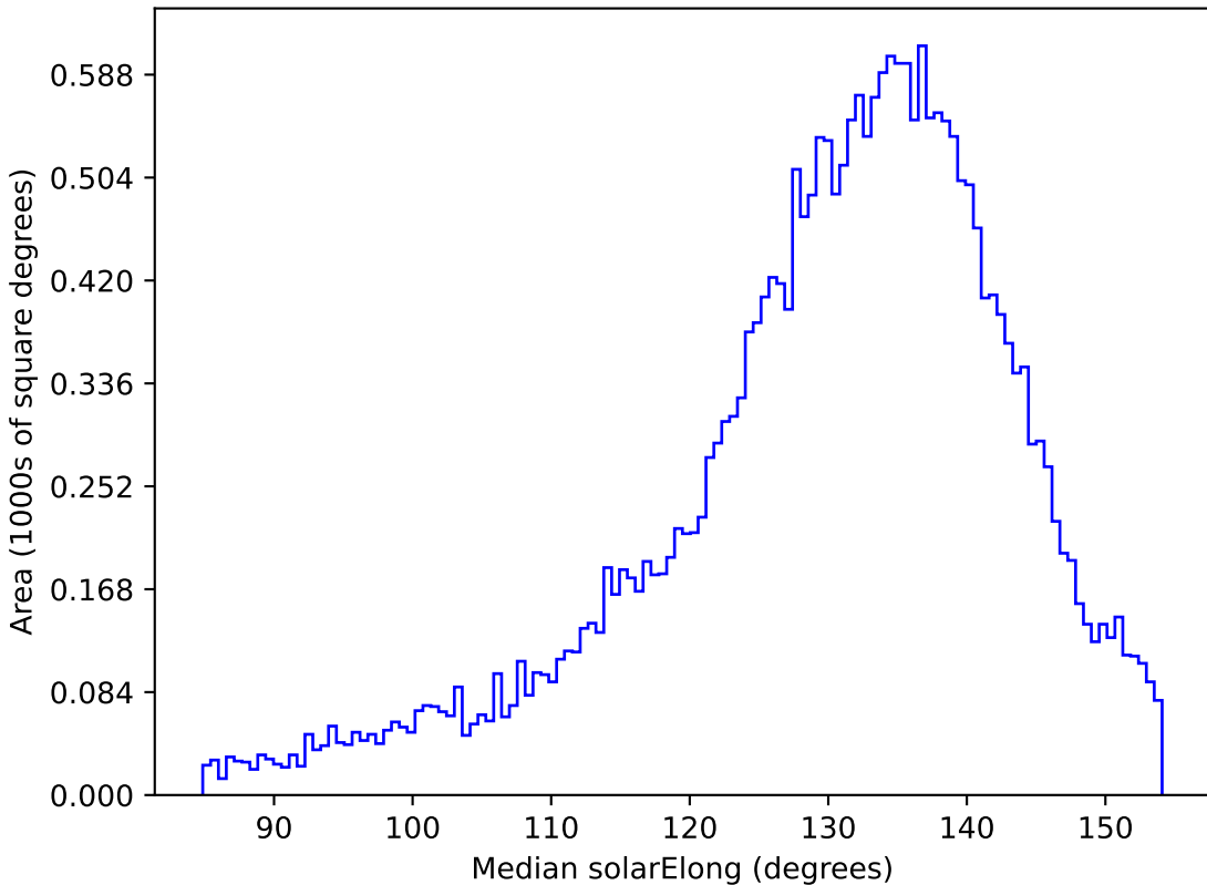
mw_roll_all_v3.3_10yrs All sky r band: Median solarElong
