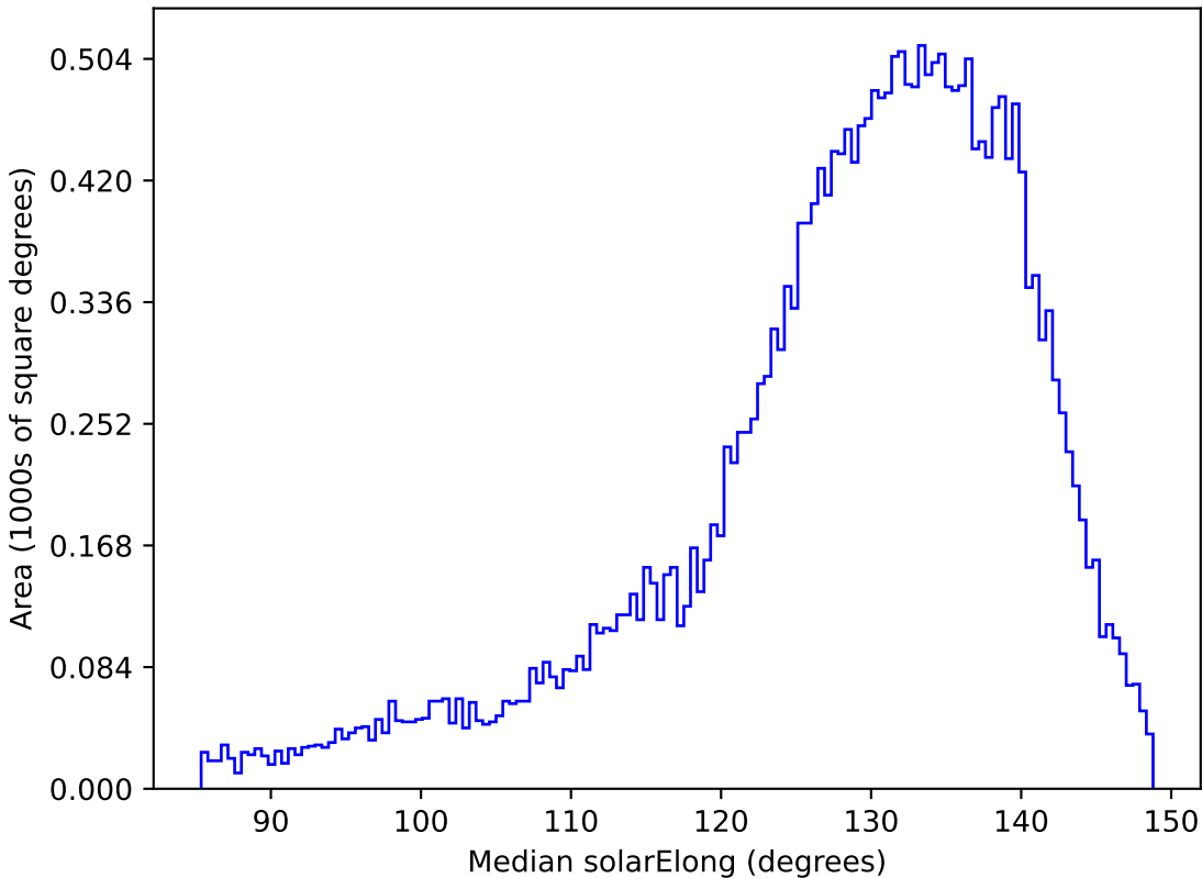
mw_roll_all_v3.3_10yrs All sky i band: Median solarElong
