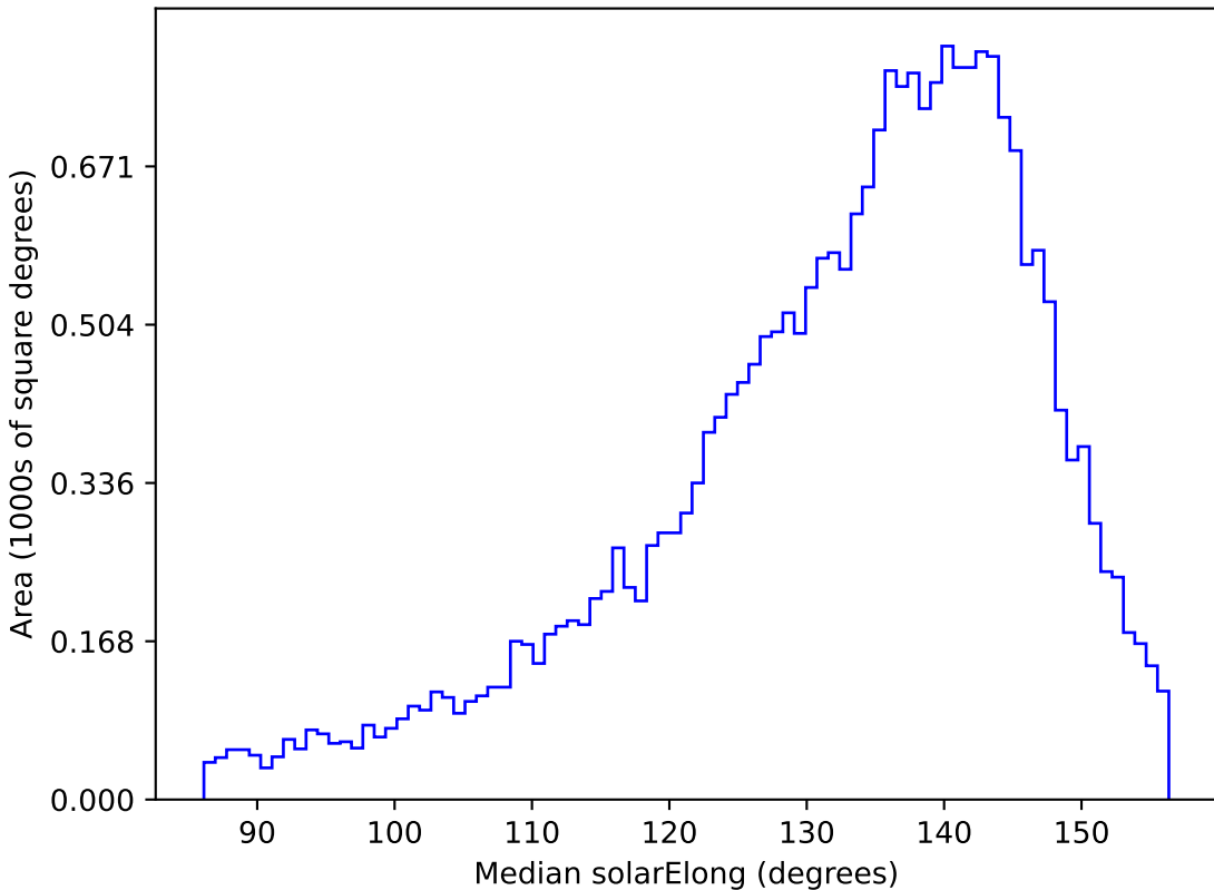
mw_roll_all_v3.3_10yrs All sky g band: Median solarElong
