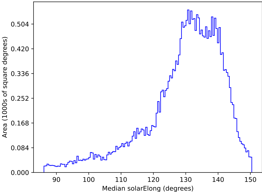
mw_roll_all_v3.3_10yrs All sky all bands: Median solarElong
