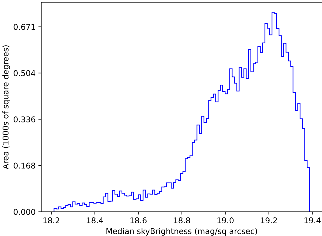
mw_roll_all_v3.3_10yrs Yr 1 z band: Median skyBrightness
