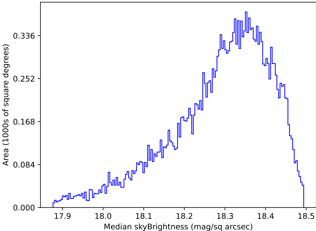
mw_roll_all_v3.3_10yrs Yr 1 y band: Median skyBrightness
