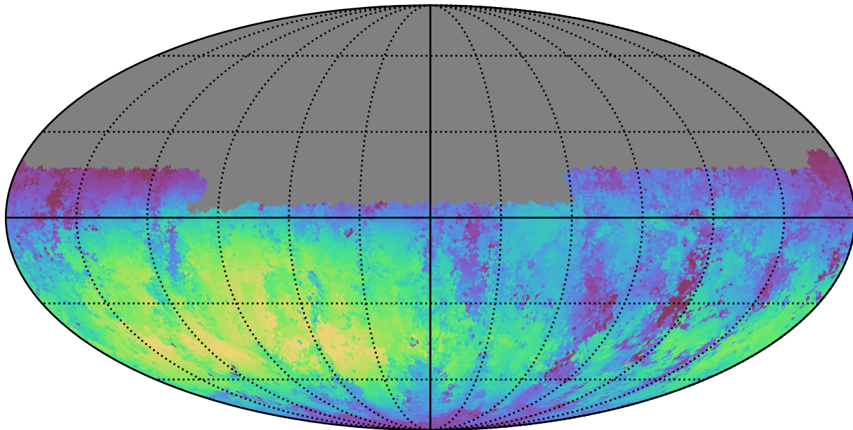
mw_roll_all_v3.3_10yrs Yr 1 u band: Median skyBrightness
